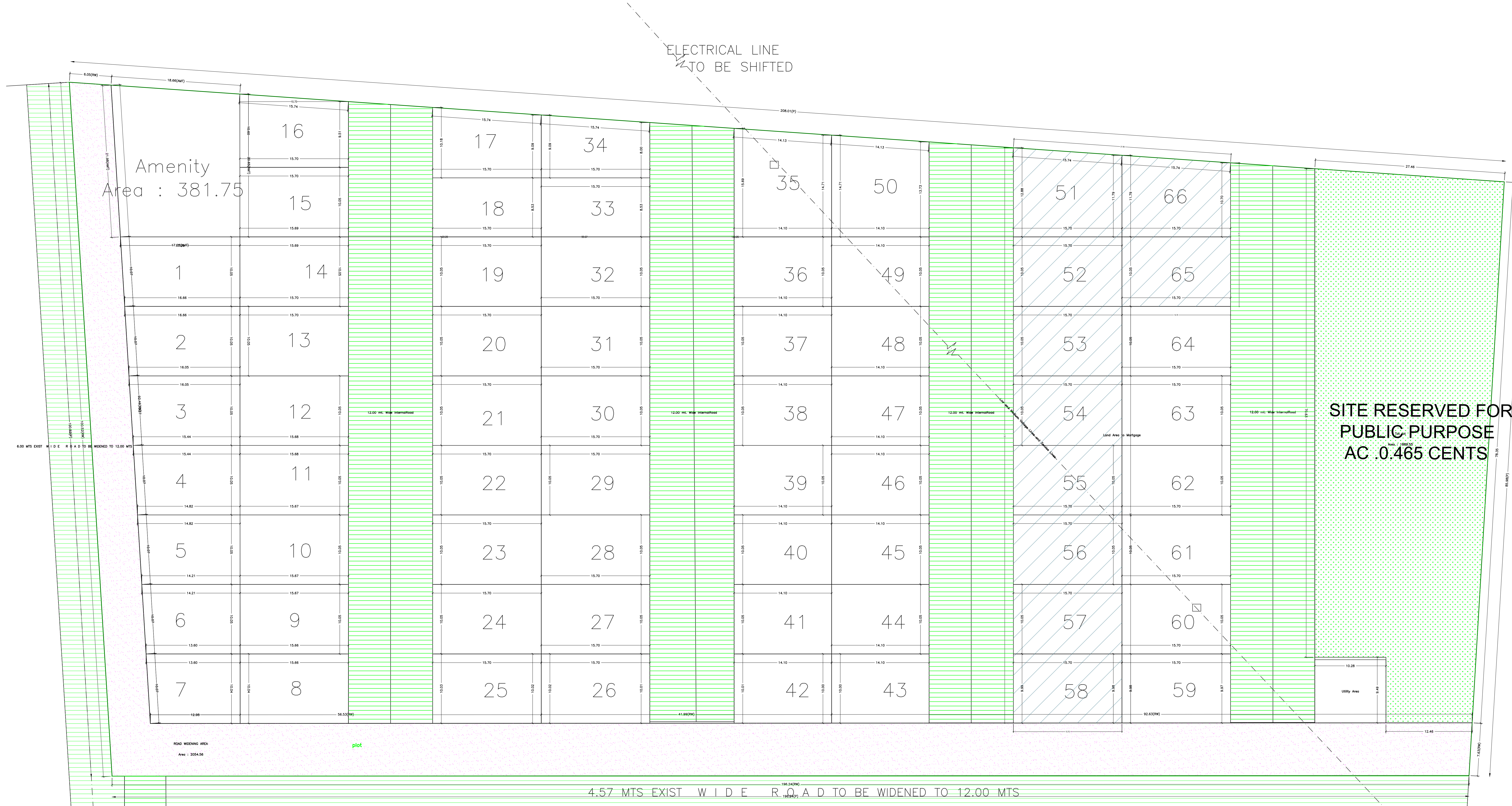
layout plan (Scale - 1:200)
